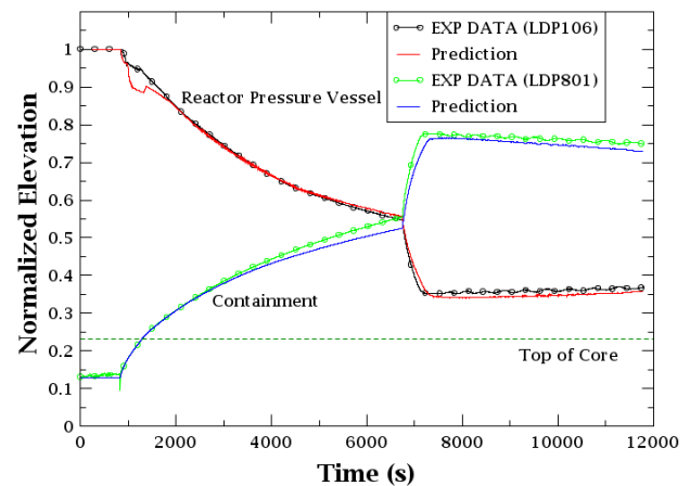
Fig. 3 Comparison of normalized experimental RPV and containment collapsed liquid level with NRELAP code predictions for blowdown event.
