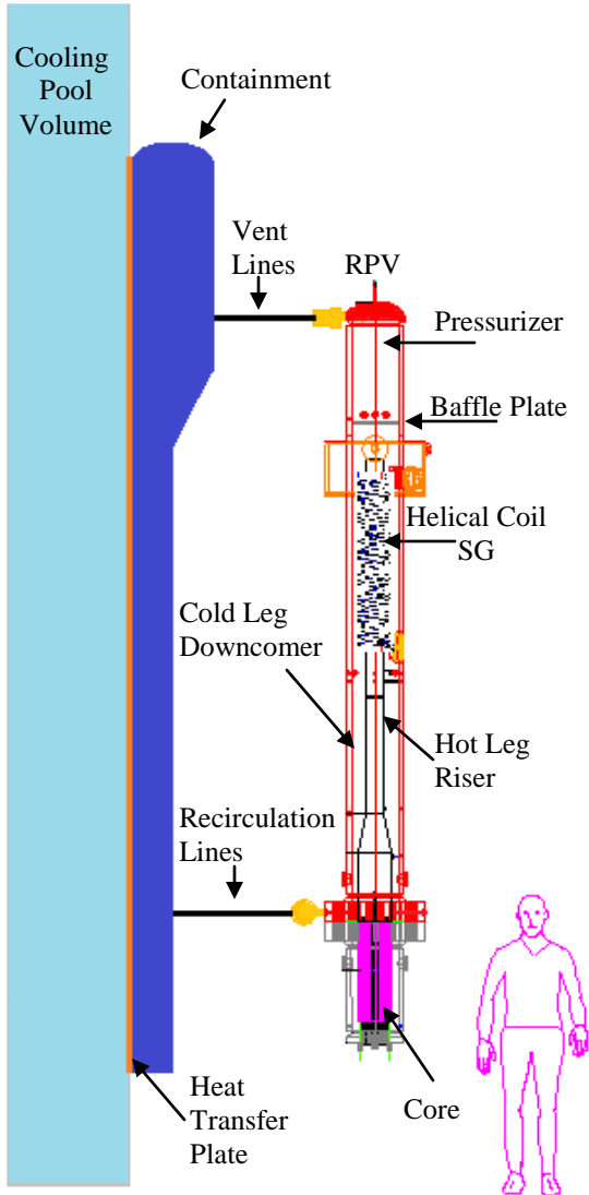
Fig. 1 Schematic of the NuScale Integral System Test (NIST) facility and major components.
