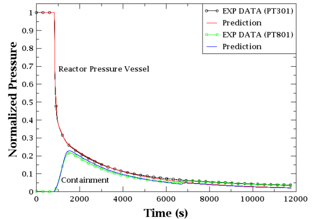
Fig. 2 Comparison of normalized experimental RPV and containment pressure with NRELAP code predictions for blowdown event.
